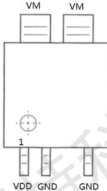
Figure 2 .Pin Configuration
